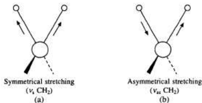
Fig. 3.2 Stretching vibrations of a \text{CH}_2 group ( \nu\text{CH}_2 )
