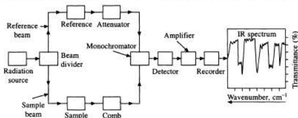
Fig. 3.1 Schematic diagram of a double-beam infrared spectrophotometer
