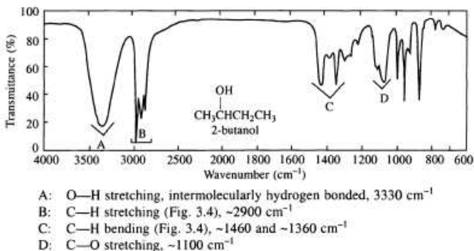
Fig. 3.7 IR spectrum of 2-butanol, neat
